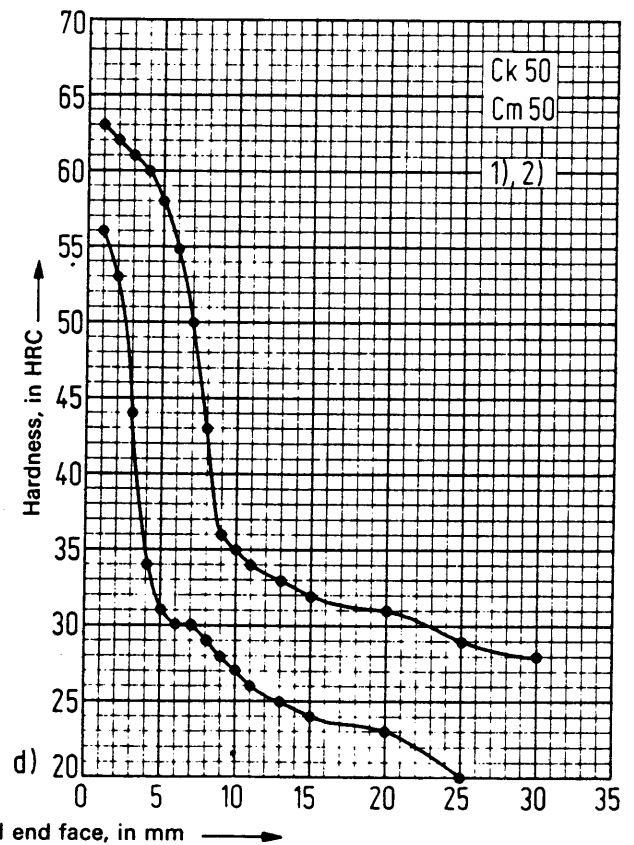
Figure 1. Scatterbands for Rockwell C hardness determined by the end quench test (The curves shown in figures 1a to 1k are provisional.)
